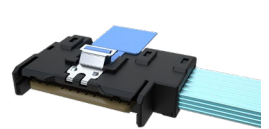
8X/74Pos-RSE (Right Side Exit w/ Pull Tab)
