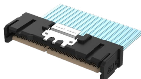
16X/124Pos-STR (Straight)
