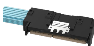
16X/124Pos-LSE (Left Side Exit)
