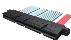
SFF-TA-1002 4C+ Receptacle (Straight w/ Ear Hole)
