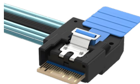
4X/38Pos-LSE (Left Side Exit)
