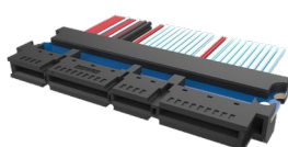
SFF-TA-1002 4C+ Receptacle (Straight)
