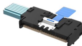
16X/124Pos-LSE (Left Side Exit w/ Pull Tab)
