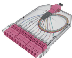
Patch Cassette
