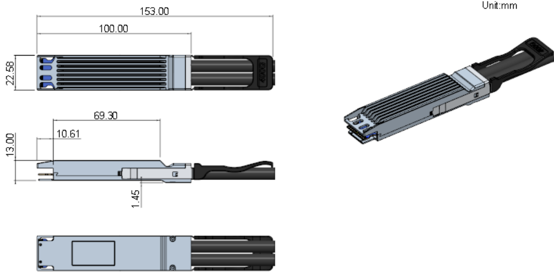
Figure 4 OSFP Form Factor
