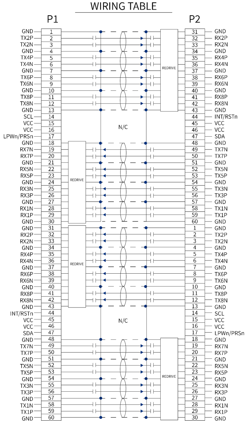
Figure 2 OSFP 800G Active Redriver Cable Assembly Wiring
