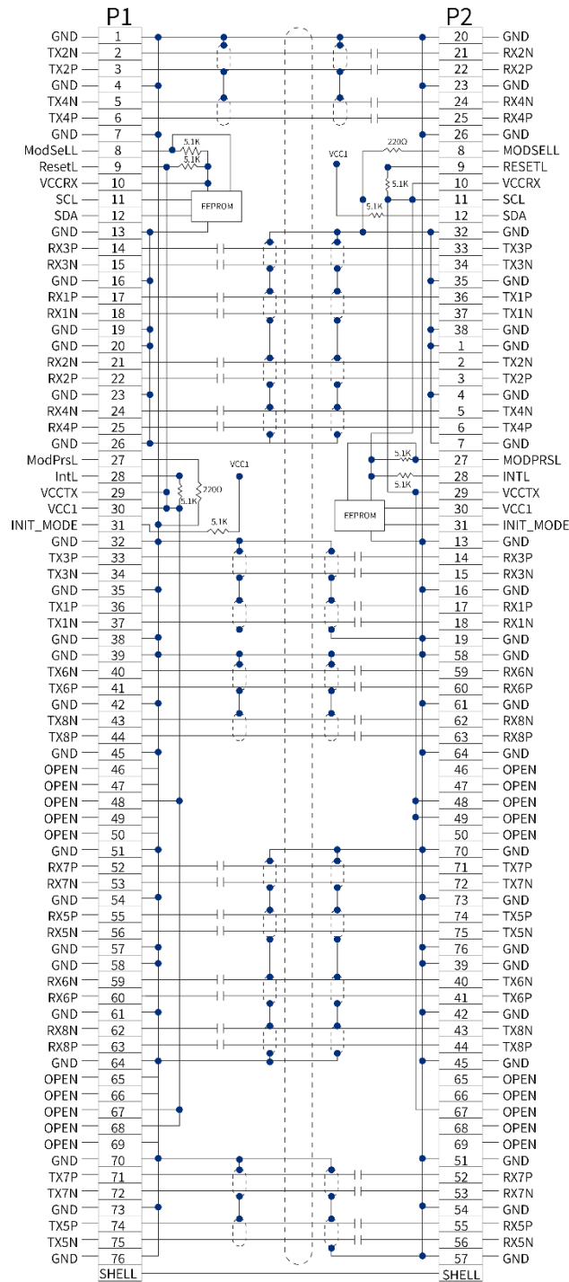
Figure 2 QSFP-DD to QSFP-DD 400G Active Redriver Cable Assembly Wiring
