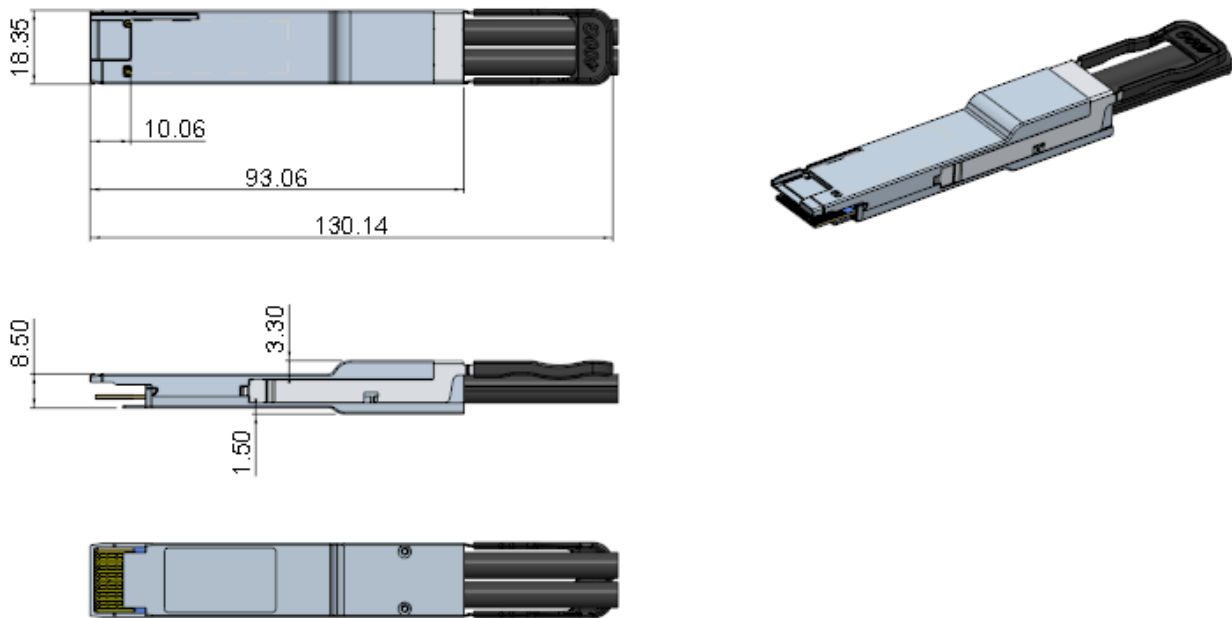
Figure 4 QSFP-DD 400 Form Factor
