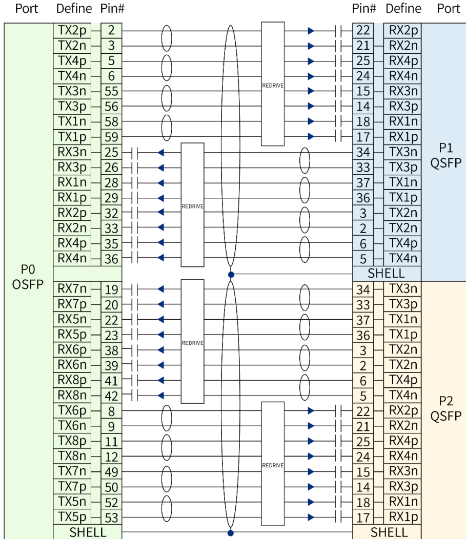
Figure 3 OSFP 400G to 2*QSFP56 Active Redriver cable Wiring
