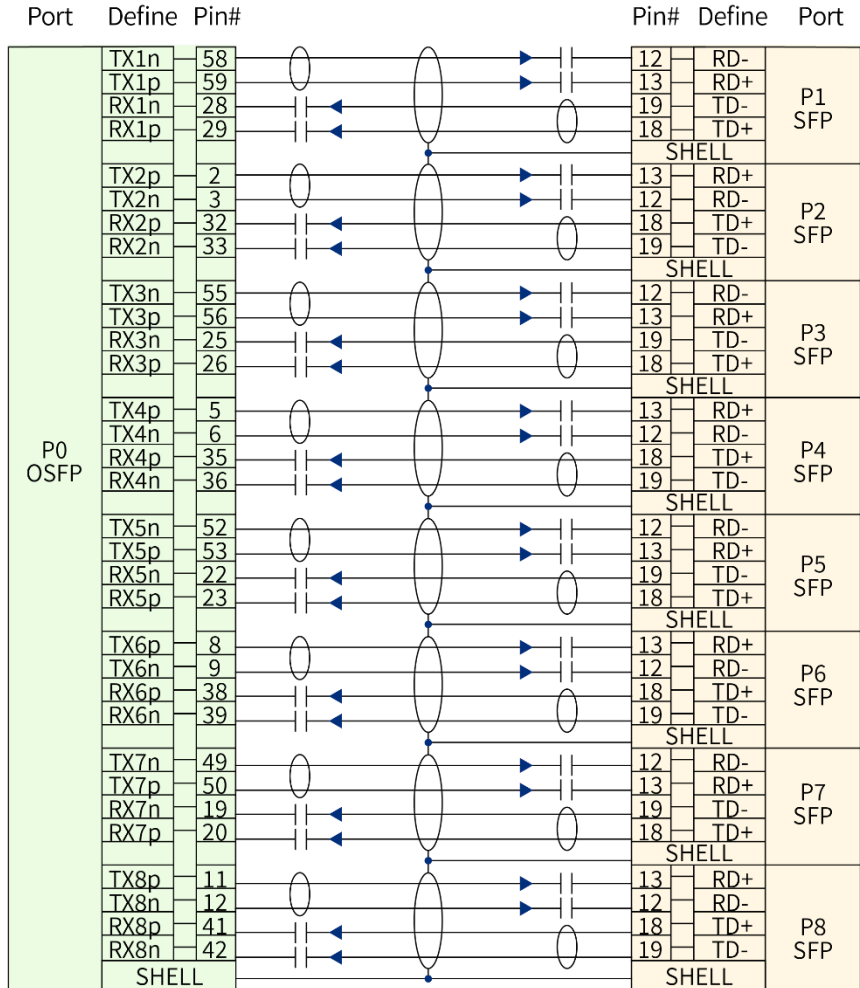
Figure 3 OSFP 400G to 8*SFP56 Direct Attached cable Wiring
