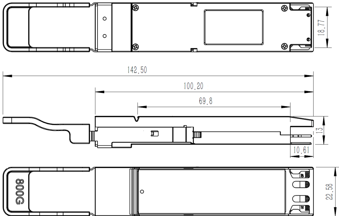
Figure 2 – Mechanical Dimensions
